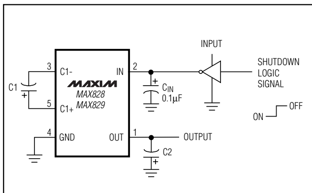
Figure 8. Shutdown Control
