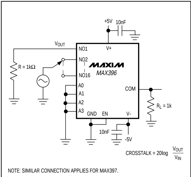
Figure 7. Crosstalk (VCT)
