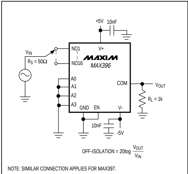
Figure 6. Off-Isolation (VISO)
