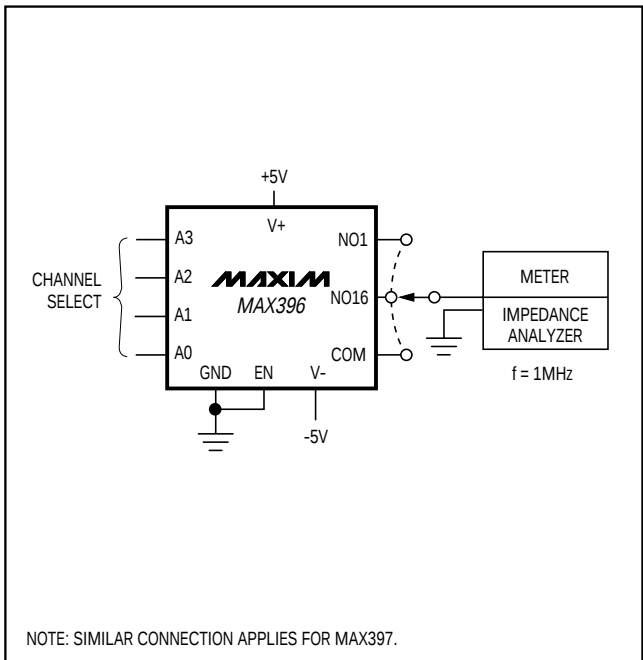
Figure 8. NO/COM Capacitance
