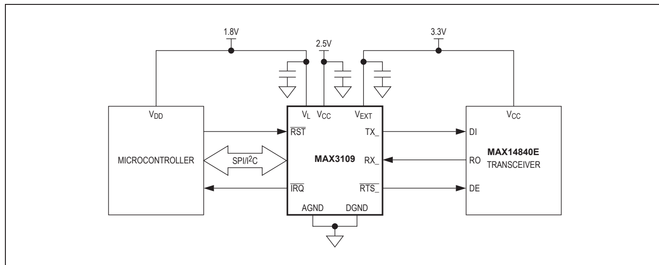
Figure 28. Logic-Level Translation
