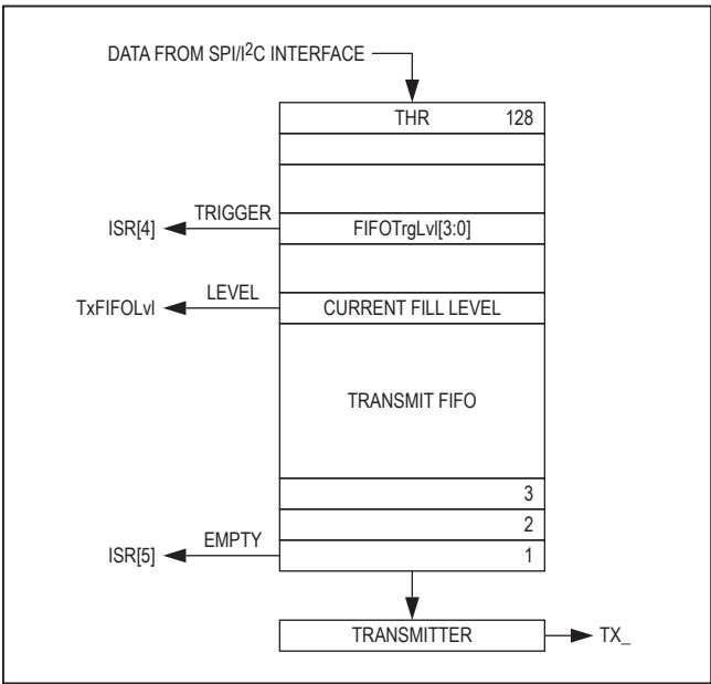
Figure 3. Transmitter FIFO Signals
