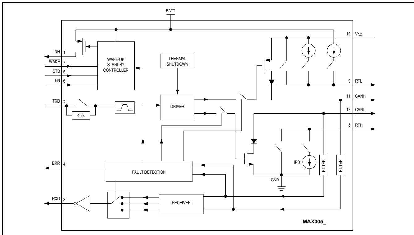
Figure 5. Block Diagram
