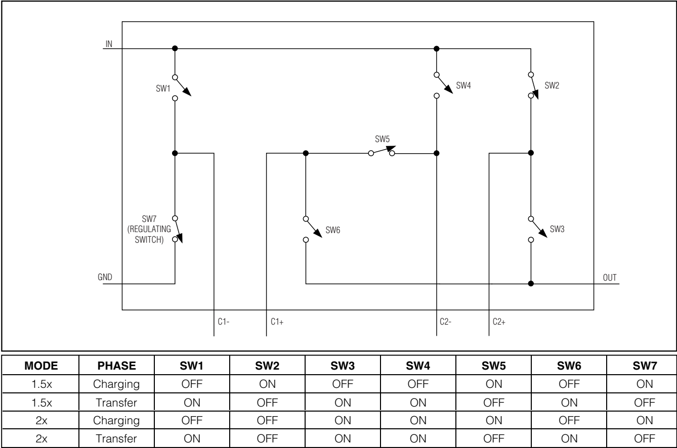
Figure 1. Functional Charge-Pump Switch Diagram (Switches Shown for 1.5x Charging Phase)
