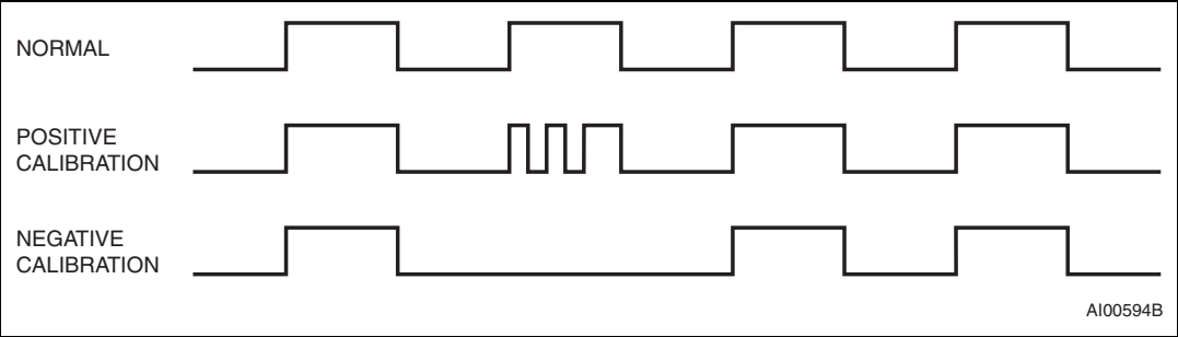
Figure 11. Clock calibration
