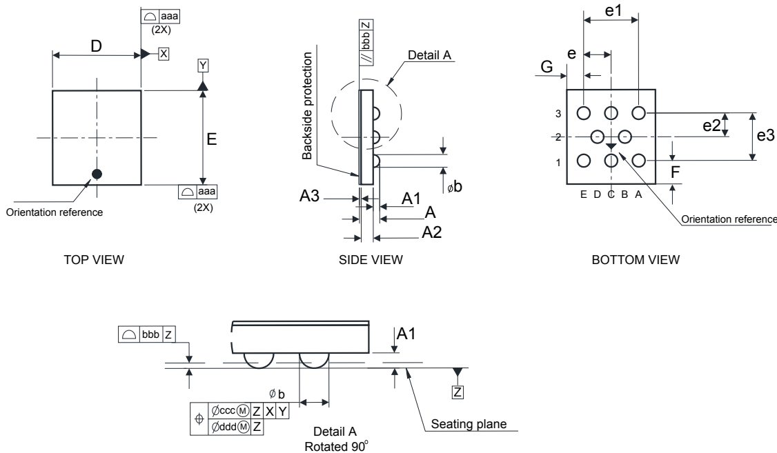
Figure 23. WLCSP8 - Outline
