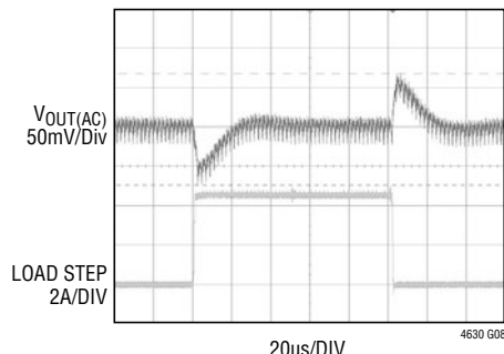
1.8V Single Phase Output Load Transient Response
