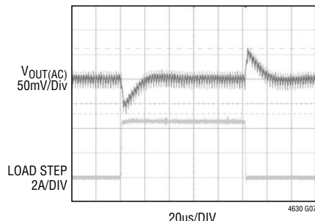
1.5V Single Phase Output Load Transient Response
