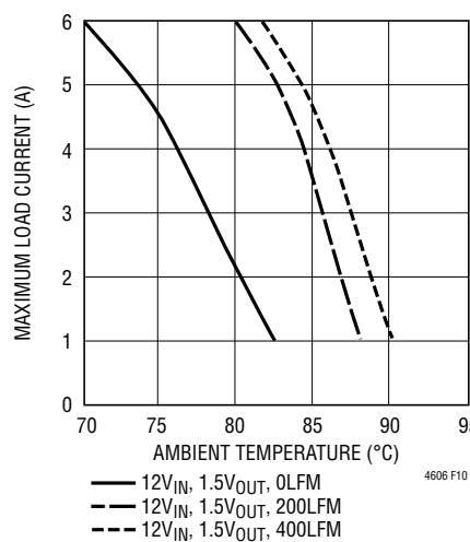
Figure 10. No Heat Sink
