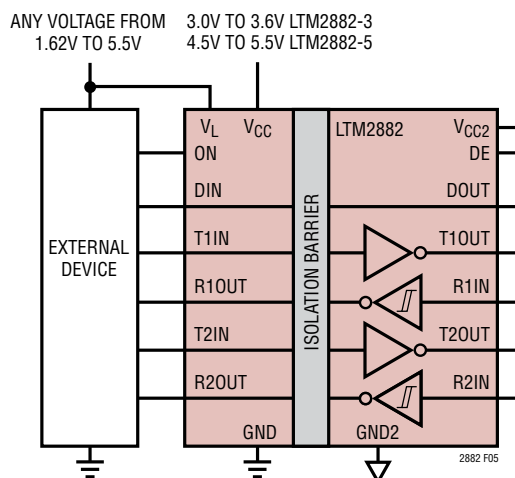
Figure 5. V_{CC} and V_I Are Independent
