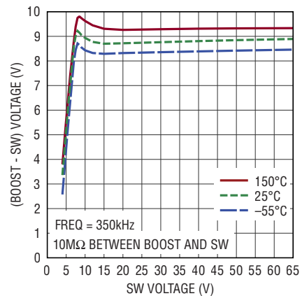
Boost Charge Pump Voltage vs SW Voltage
