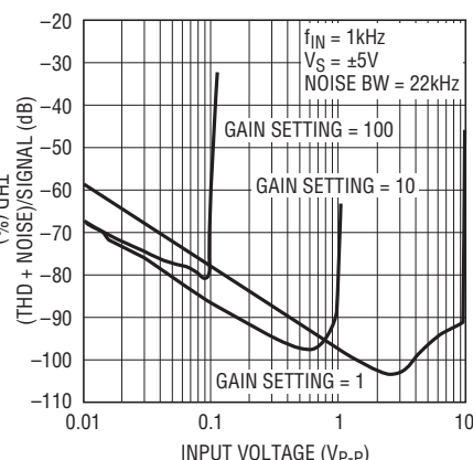
LTC6910-1 THD + Noise vs Input Voltage
