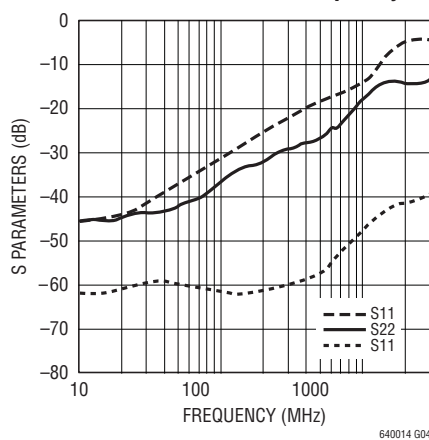
Input and Output Reflection and Reverse Isolation vs Frequency
