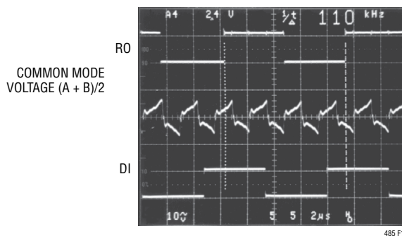
Figure 17. System Common Mode Voltage at 110kHz
