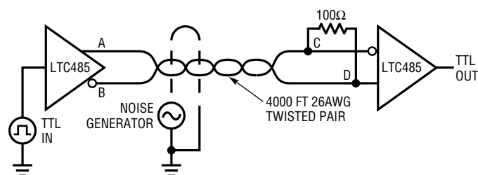
Figure 14. Line Length Test Circuit
