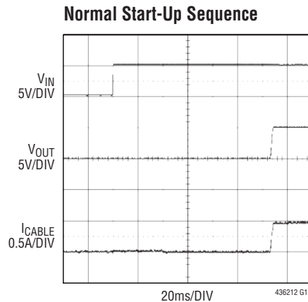
FIGURE 4 CIRCUIT R_{IN} = 150\text{m}\Omega , L_{IN} = 0.7\mu\text{H} \text{LOAD} = 10\Omega , C_{OUT} = 10\mu\text{F}
