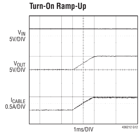
FIGURE 4 CIRCUIT R_{IN} = 150\text{m}\Omega , L_{IN} = 0.7\mu\text{H} \text{LOAD} = 10\Omega , C_{OUT} = 10\mu\text{F}
