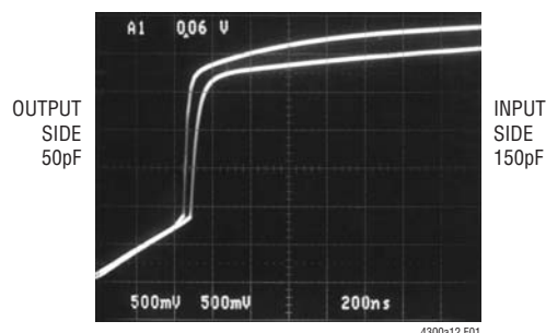
Figure 1. Input-Output Connection t_{PHL}
