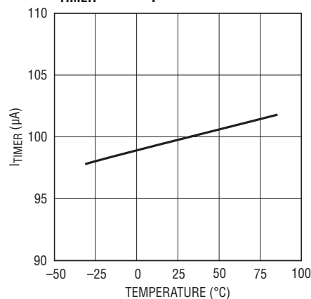
I_{TIMER} vs Temperature
