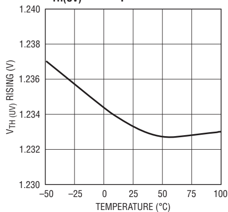
V_{TH(UV)} vs Temperature
