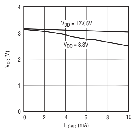
INTV_{CC} vs I_{LOAD}
