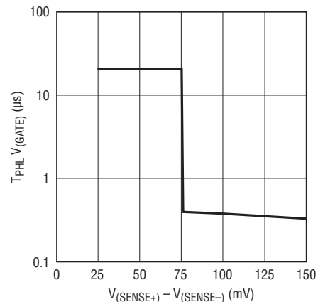
T_{PHL(GATE)} vs Sense Voltage
