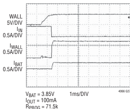
WALL Connect Waveforms, V_{IN} = 5V
