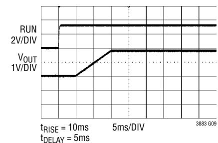
Soft-Start Ramp
