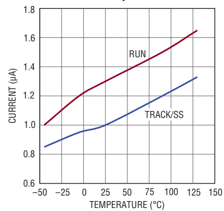
RUN and TRACK/SS Pull-Up Currents vs Temperature
