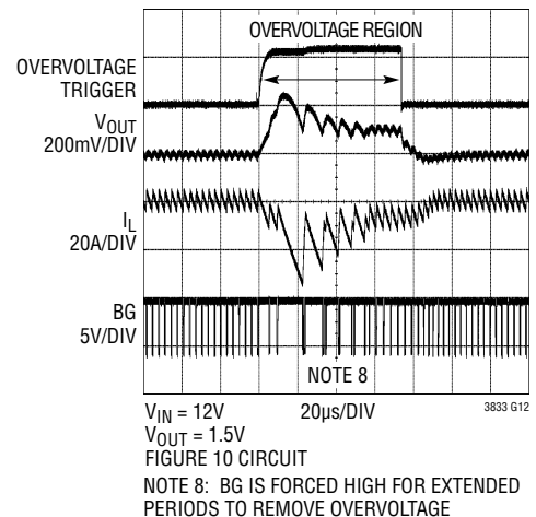
Overvoltage Protection
