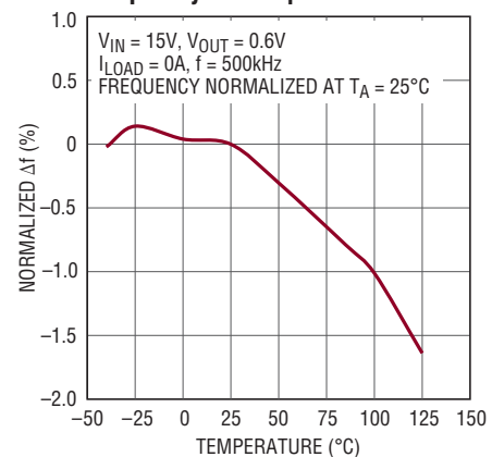
Non-Synchronized Switching Frequency vs Temperature
