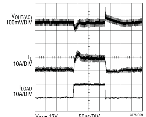
Load Step in Pulse-Skipping Mode
