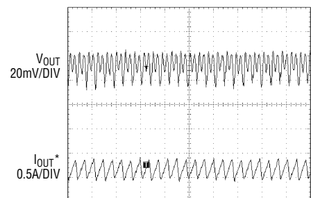
Constant Frequency (Burst Inhibit) Operation (Figure 12)
