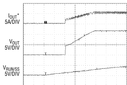
Soft-Start Up (Figure 12)
