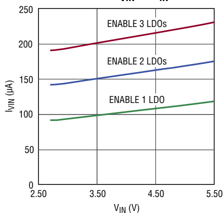
LD02 to LD04 I_{VIN} vs V_{IN}
