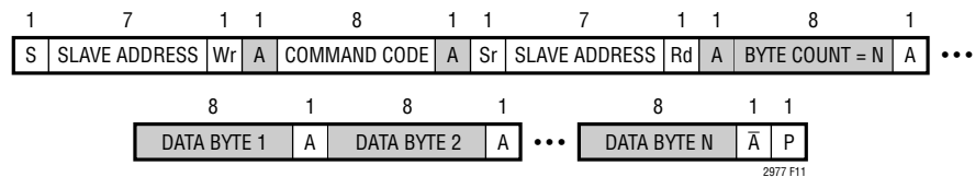
Figure 11. Block Read
