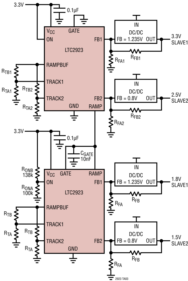
Daisy-Chained Application
