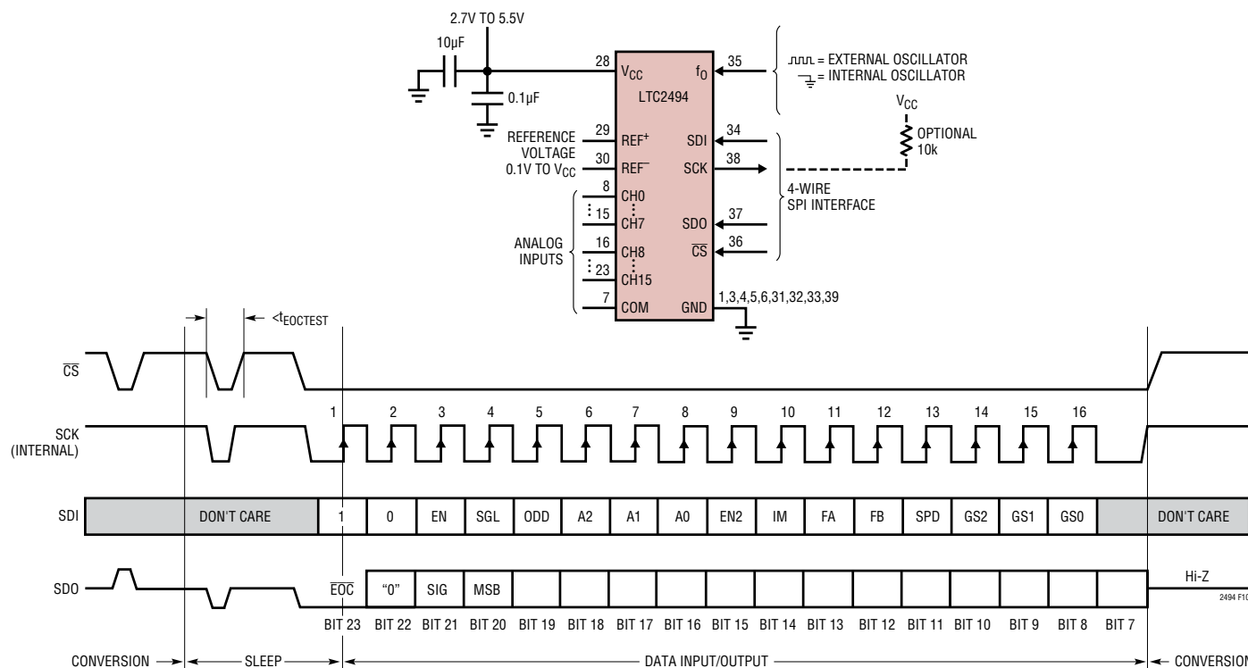
Figure 10. Internal Serial Clock, Reduced Data Output Length with Valid Channel and Configuration Selection
