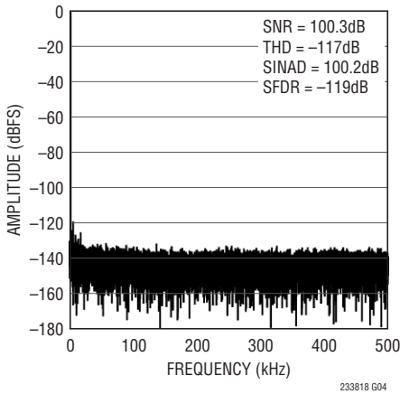
32k Point FFT f_s = 1\text{Mps} , f_{\text{IN}} = 2\text{kHz}
