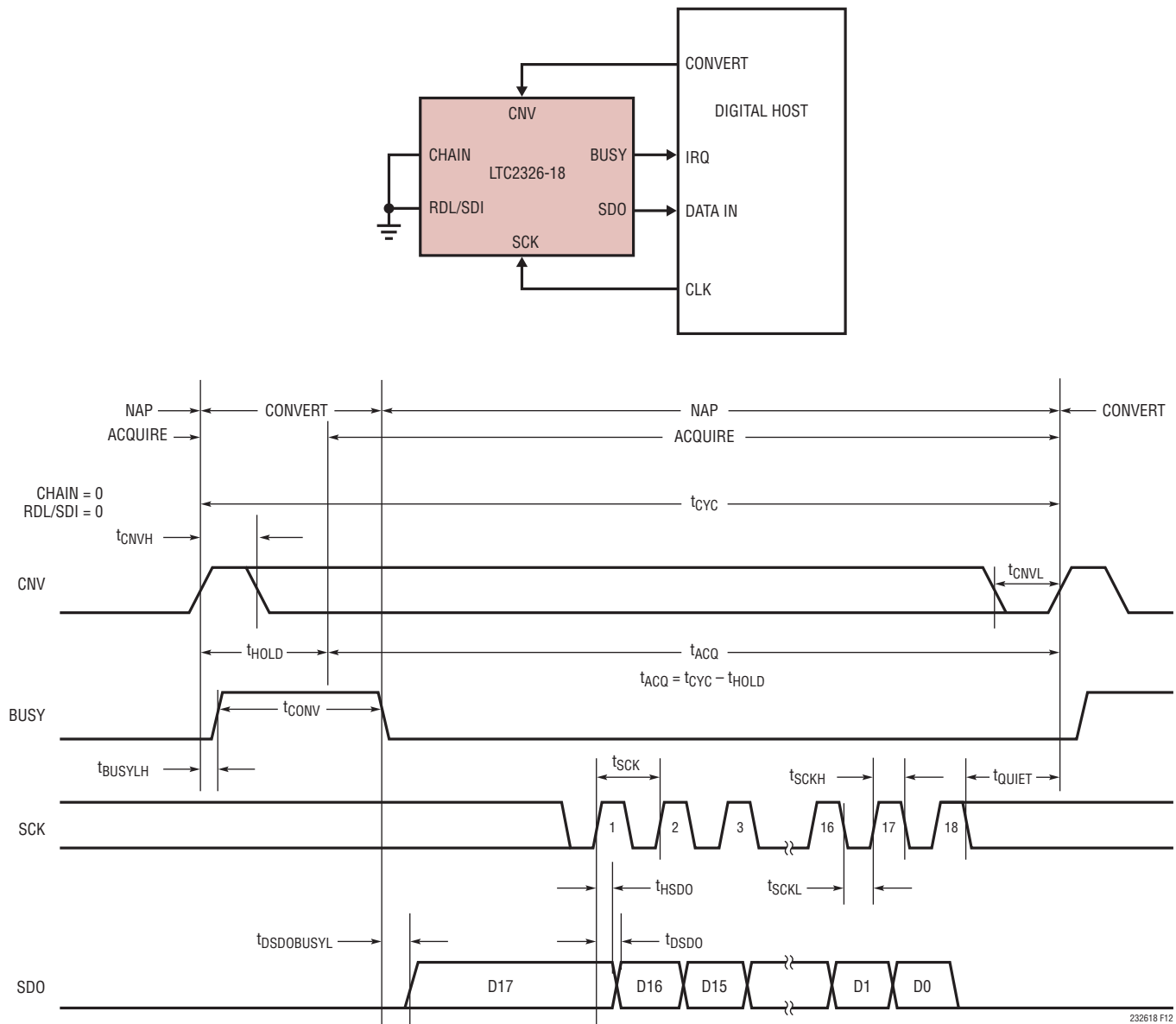
Figure 10. Using a Single LTC2326-18 in Normal Mode
