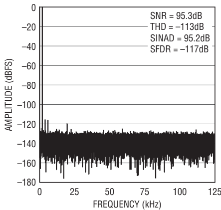
32k Point FFT f_s = 250\text{ksps} , f_{\text{IN}} = 2\text{kHz}
