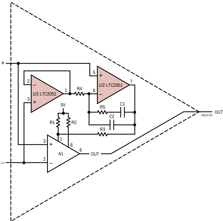
Obtaining Ultralow V_{OS} Drift and Low Noise
