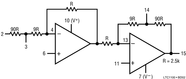
NOTE: FOR A VOLTAGE GAIN OF 10V/V SHORT PIN 2 TO 3, AND PIN 14 TO 15.
