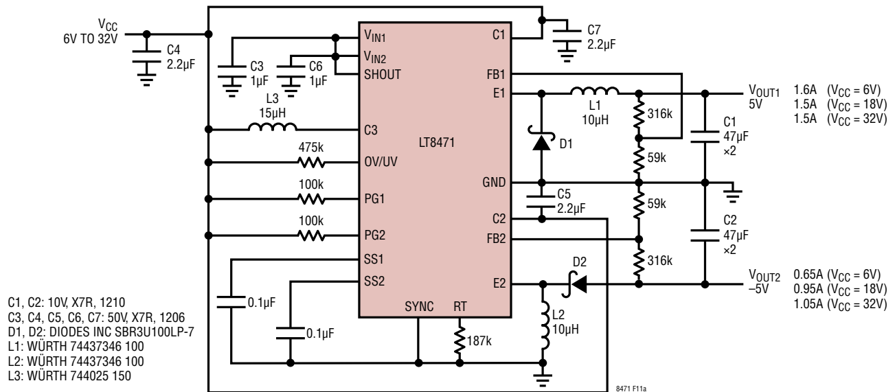
Figure 11a. Wide Input Range Converter with \pm 5\text{V} Output Voltages at 450kHz
