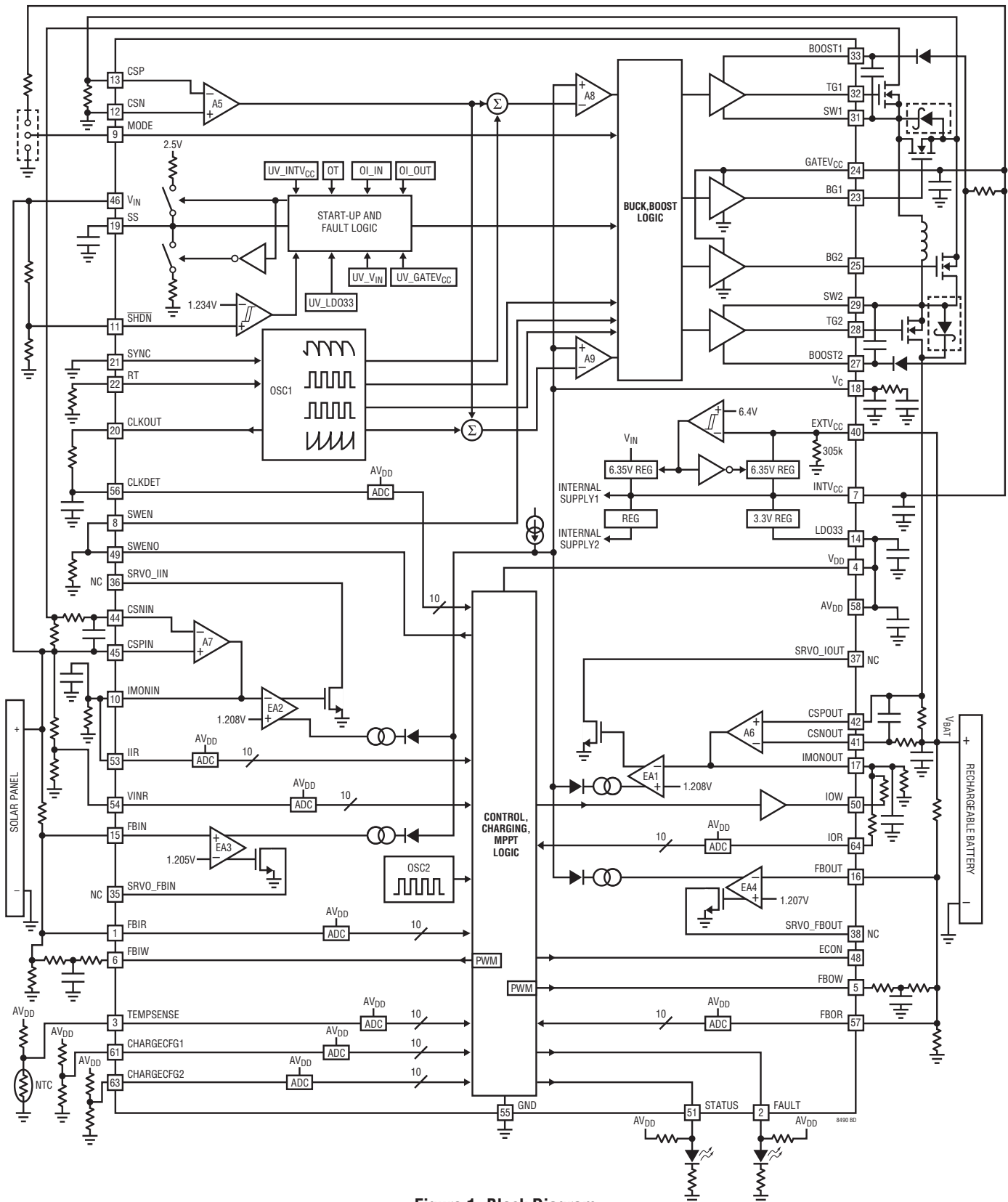
Figure 1. Block Diagram
