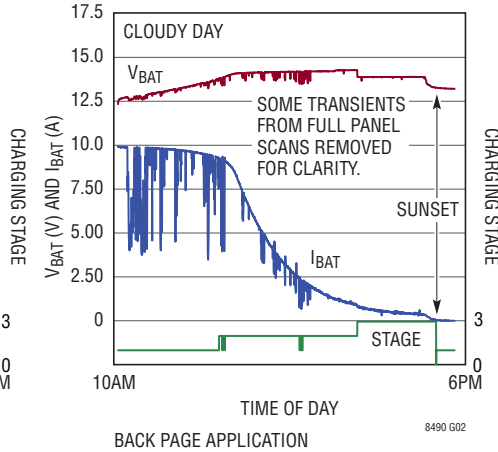
Solar Powered Charging Lead Acid Battery "B"
