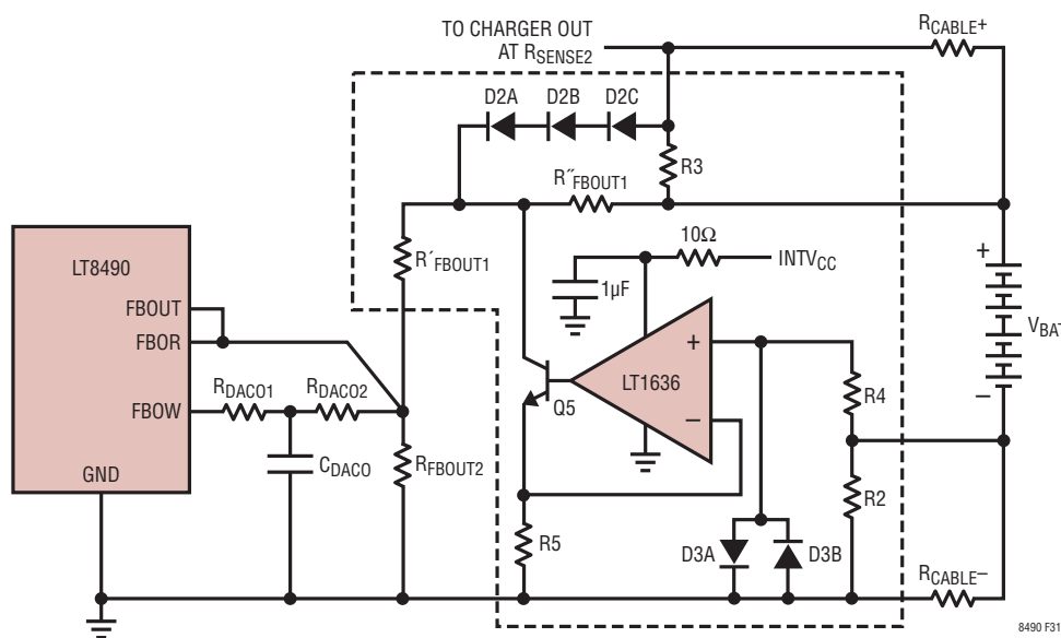
Figure 31. Remove (+) and (-) Cable V_{IB} Measurement Errors
