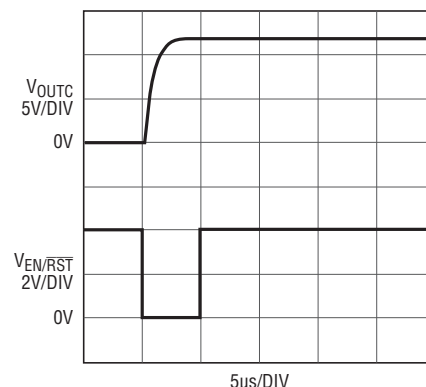
LT6108-1 Comparator Reset Response
