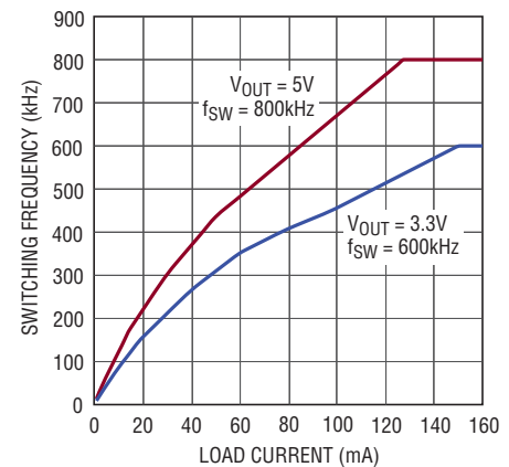
Burst Frequency
