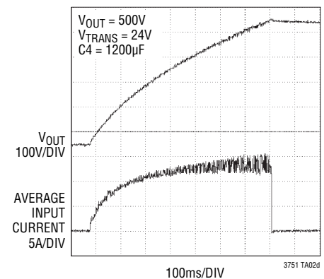
Charging Waveform
