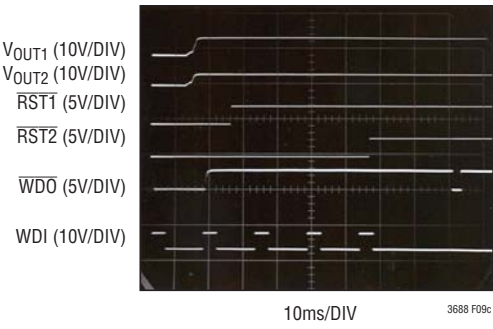
Figure 9c. CONFIG = OPEN
