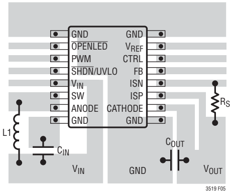
Figure 5. Suggested Layout
