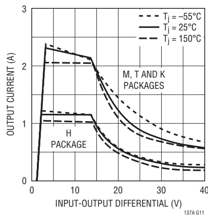
Current Limit
