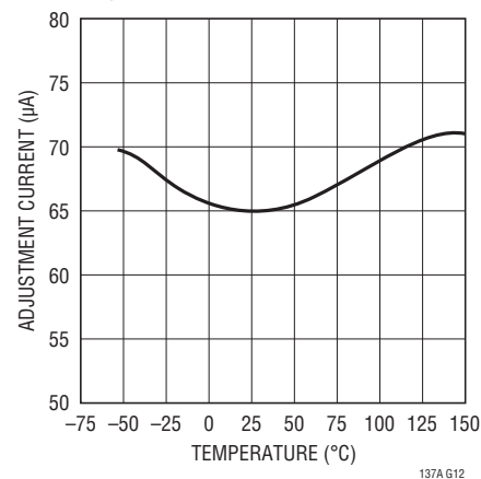
Adjustment Current
