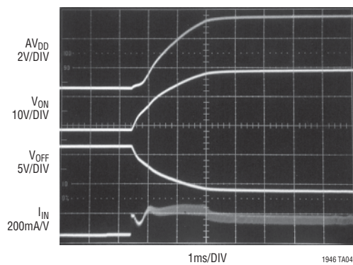
Start-Up Waveforms
