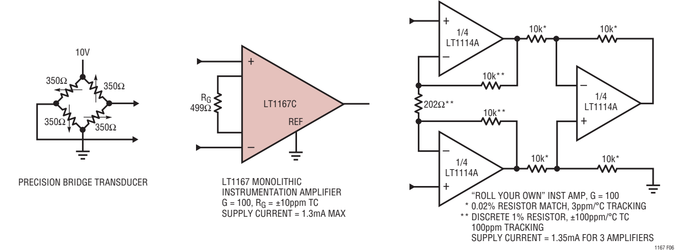
Figure 6. “Roll Your Own” vs LT1167
