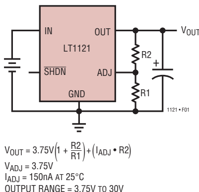
Figure 1. Adjustable Operation
