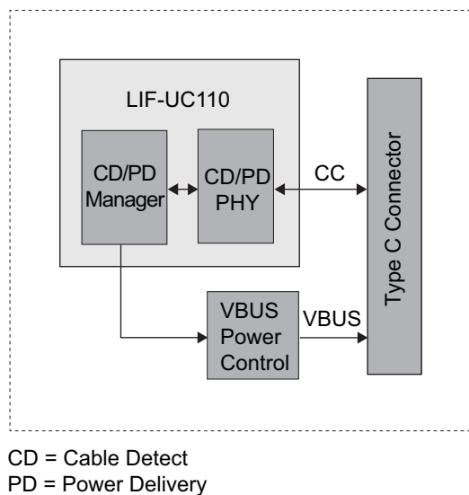
Figure 2-4. USB CD/PD Charger Solution (Non-Captive Cable) Block Diagram
