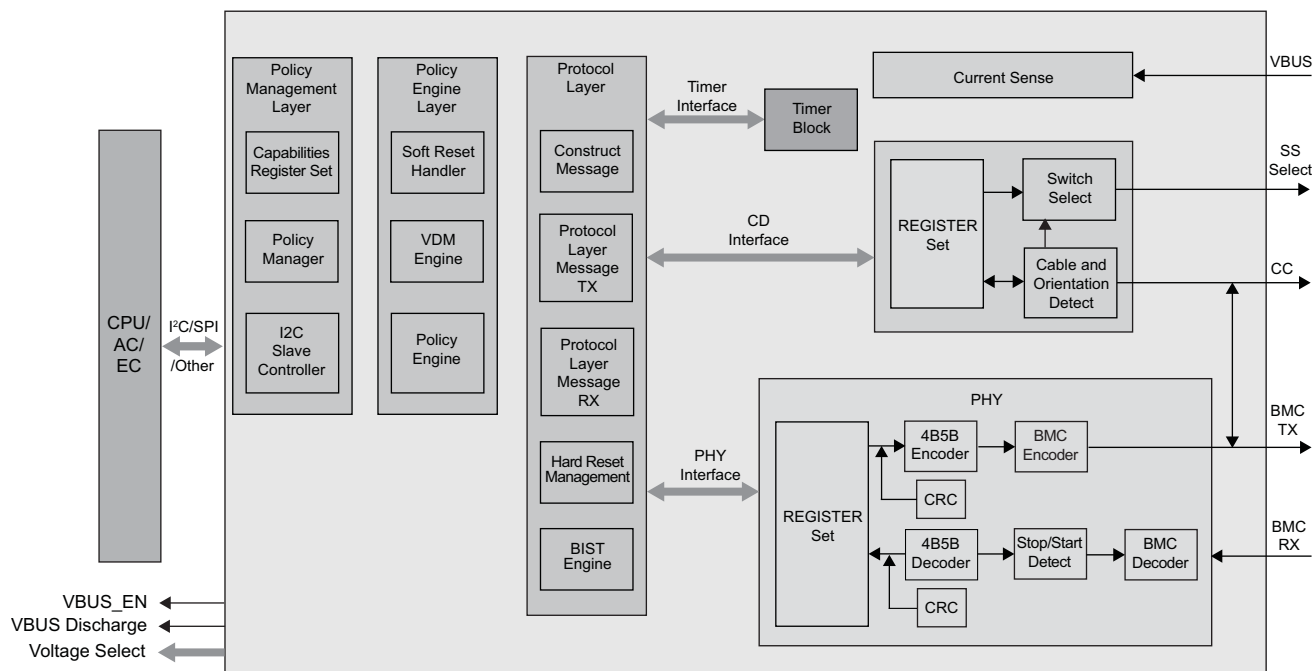
Figure 2-1. High-level Functional Block for USB Type-C Physical Layer and Power Detect Protocol
