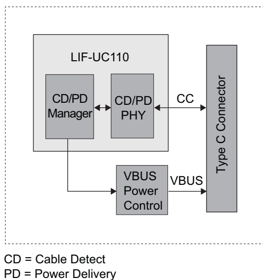
Figure 2-2. USB CD/PD Charger Solution (Captive Cable) Block Diagram
