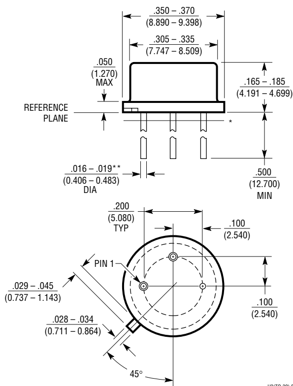
H Package 3-Lead TO-39 Metal Can (Reference LTC DWG # 05-08-1330)
