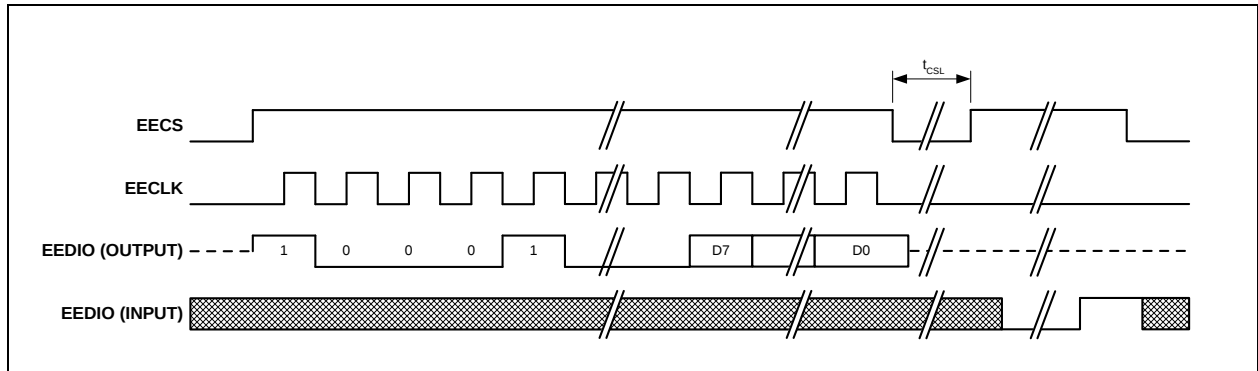
FIGURE 3-10: EEPROM WRAL CYCLE
