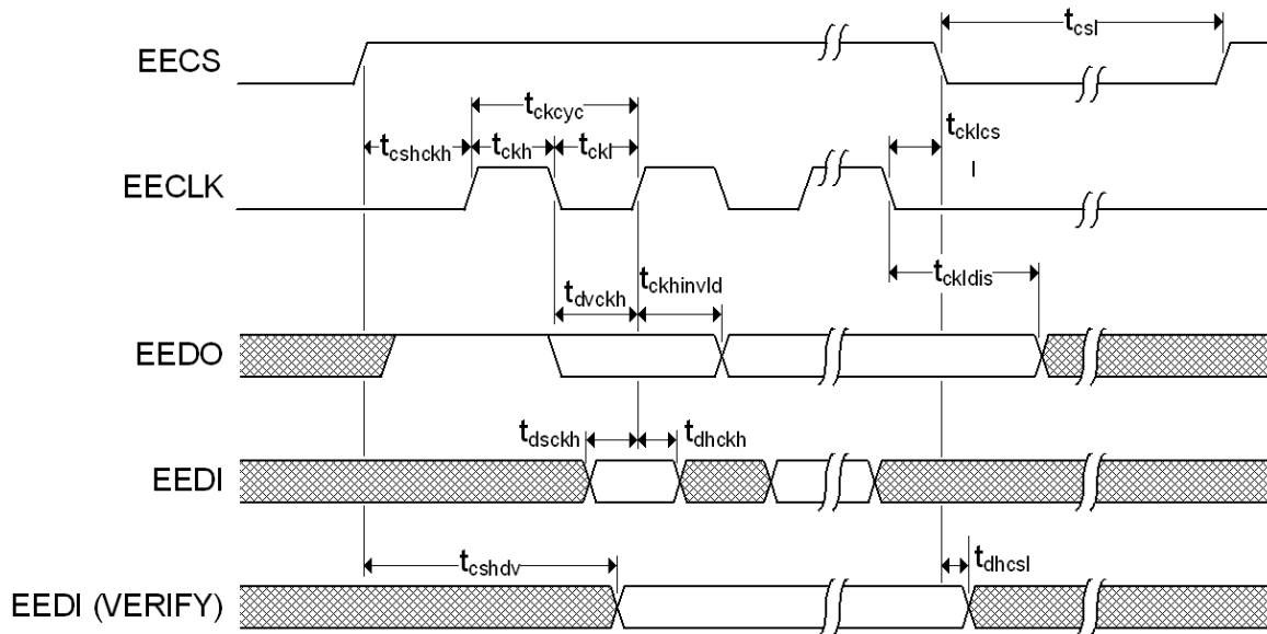
Figure 7.5 EEPROM Timing
