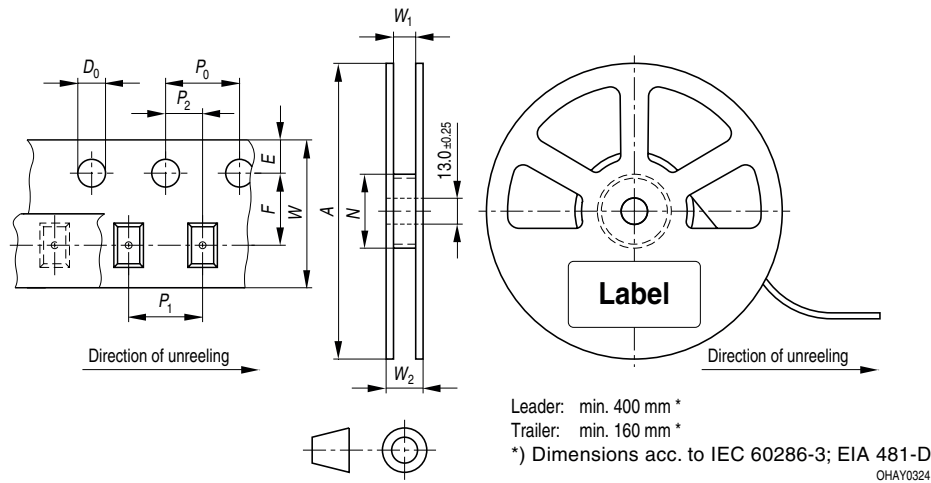
Tape dimensions in mm
