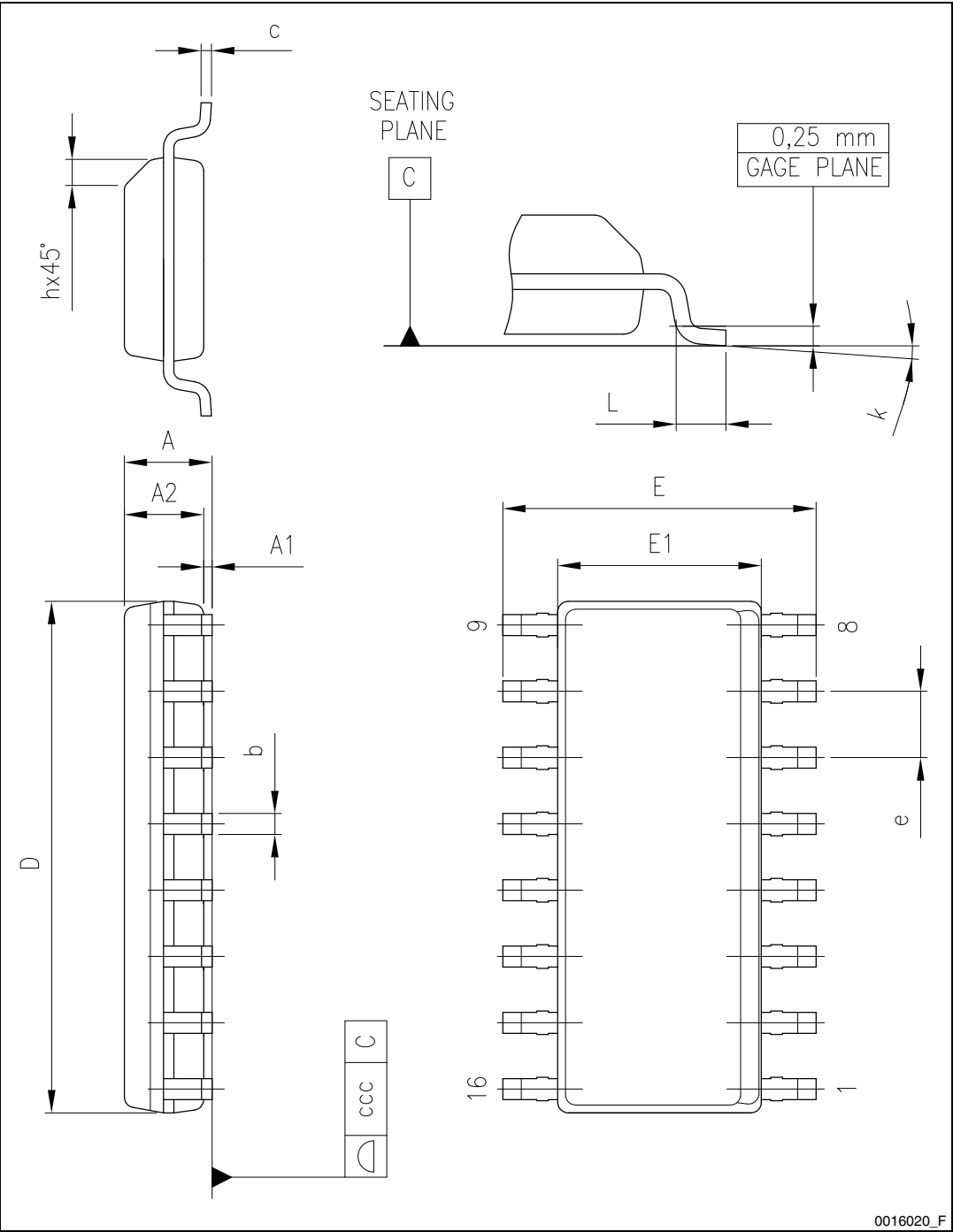
Figure 33. Package drawing
