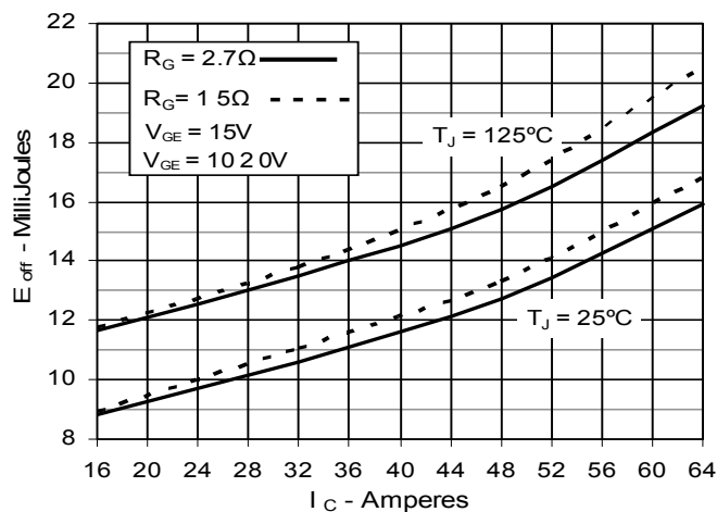
Fig. 11. Dependence of E_{off} on I_C
