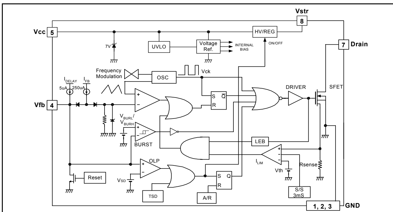
Figure 4. Functional Block Diagram of FSD200B
