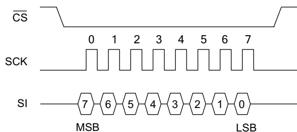
Figure 15. SPI Mode 0
