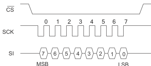
Figure 16. SPI Mode 3
